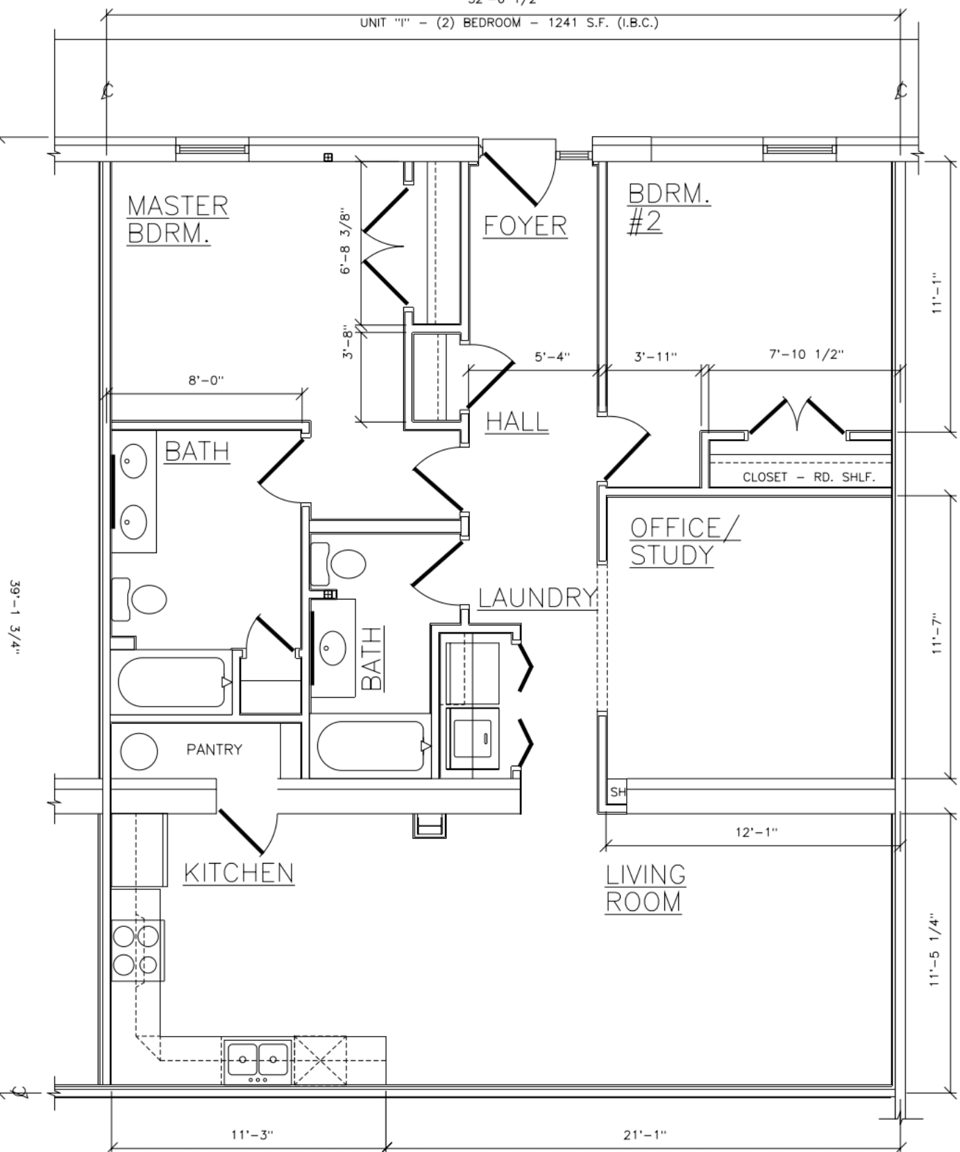
UNIT - 1 Floor Plan: 2 Bedroom - 1241 S.F.
