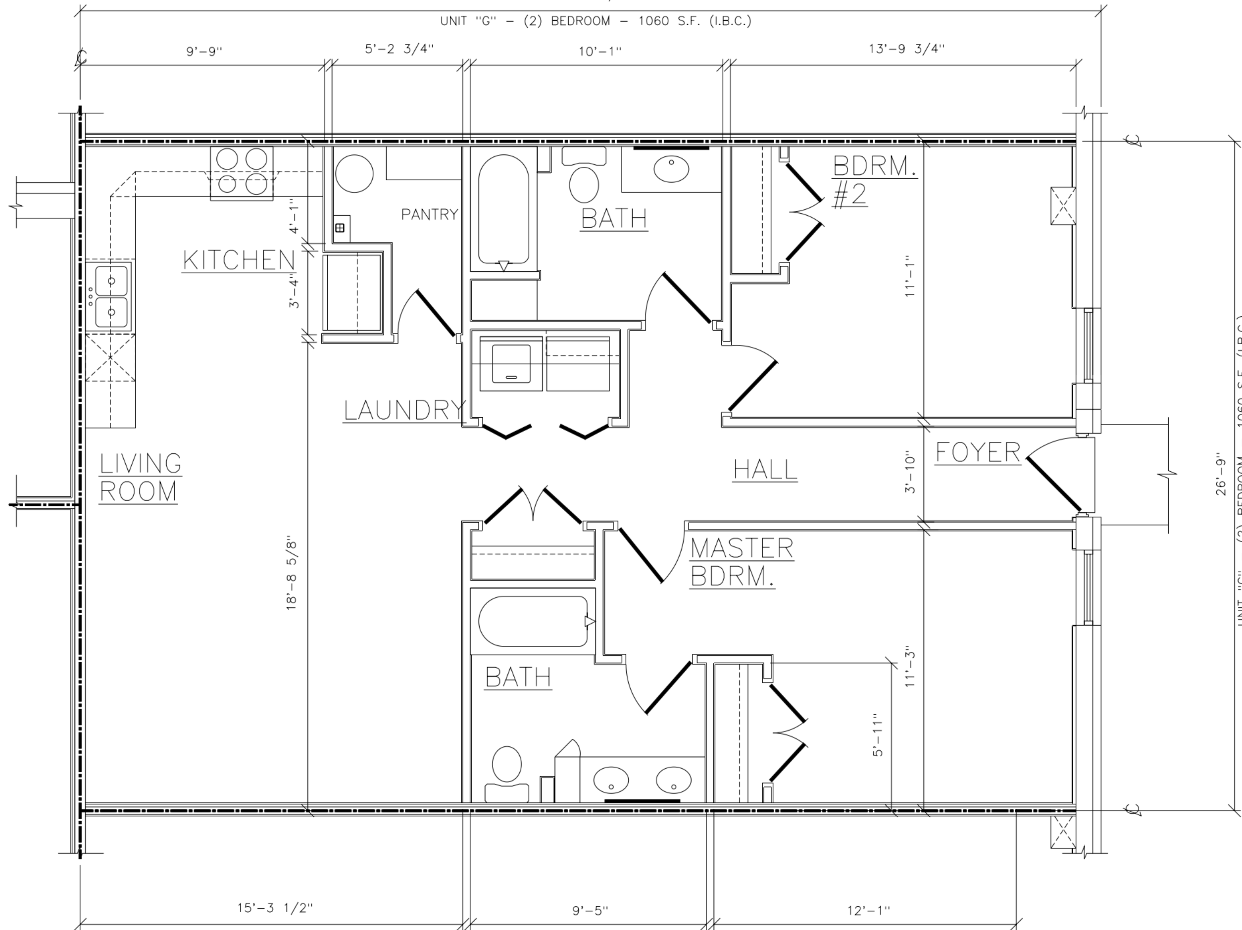
UNIT - G Floor Plan: 2 Bedroom - 1060 S.F.
