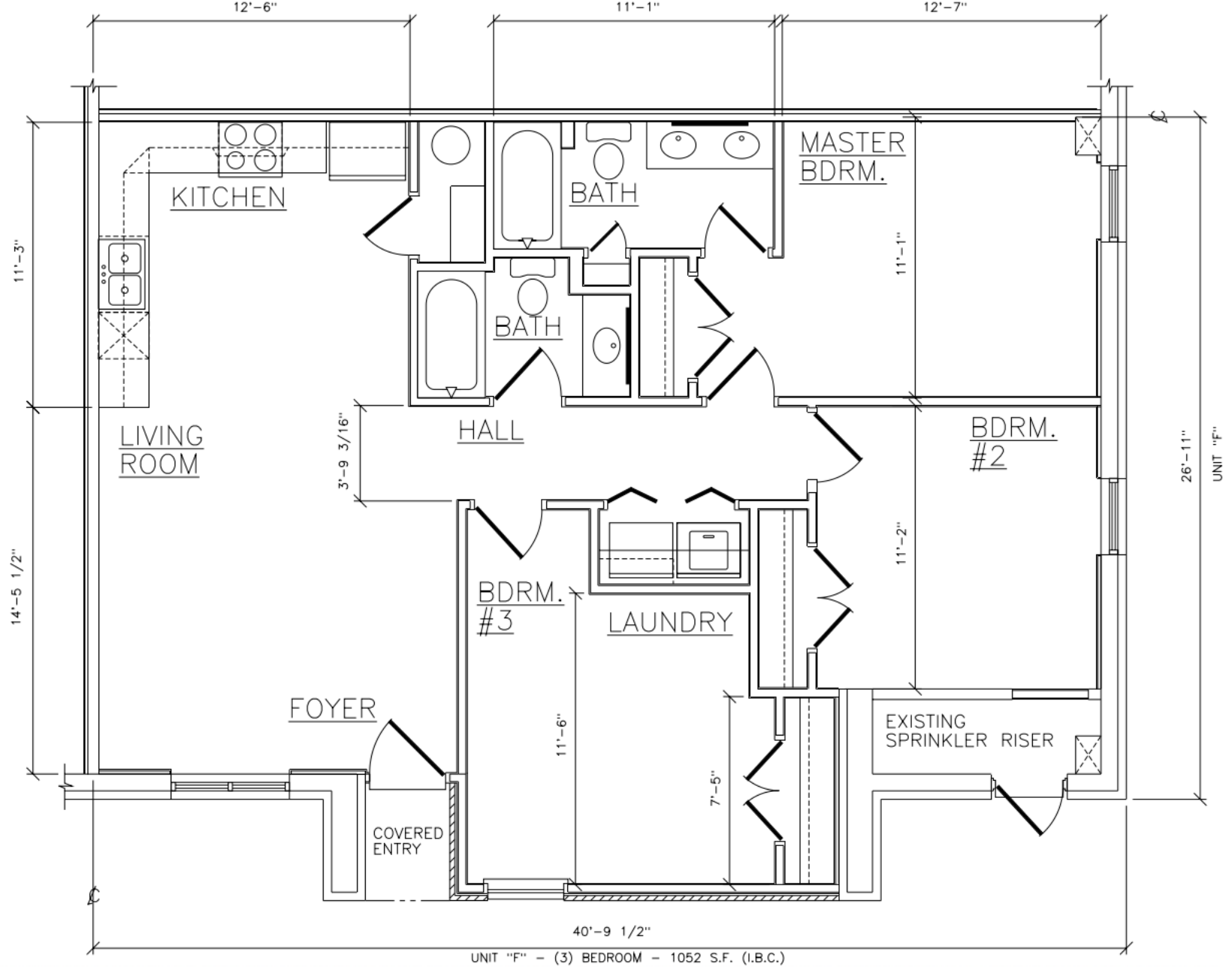
UNIT - F Floor Plan: 3 Bedroom - 1052 S.F.
